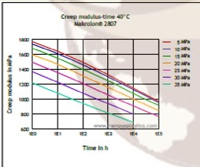
Creep modulus-time 40 °C
