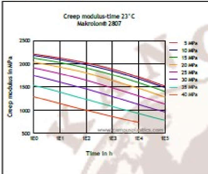
Creep modulus-time 23 °C
