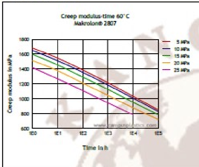
Creep modulus-time 60°C
