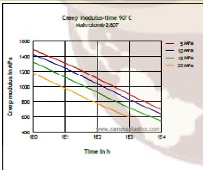
Creep modulus-time 90°C
