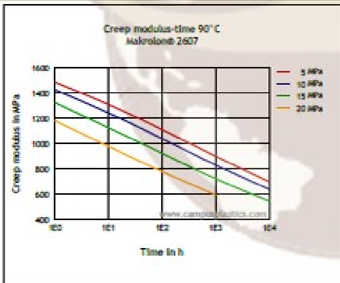
Creep modulus-time 90°C
